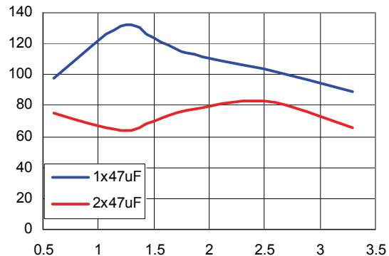
Figure 34. Input ripple voltage for various output voltages with 1x47 µF or 2x47 µF ceramic capacitors at the input (12A load). Input voltage is 5V.
