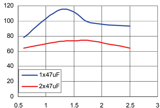
Figure 35. Input ripple voltage in mV, p-p for various output voltages with 1x47 µF or 2x47 µF ceramic capacitors at the input (12A load). Input voltage is 3.3V.
